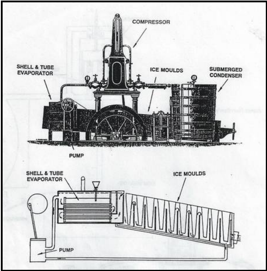
The Harrison-Siebe ice-making machine
