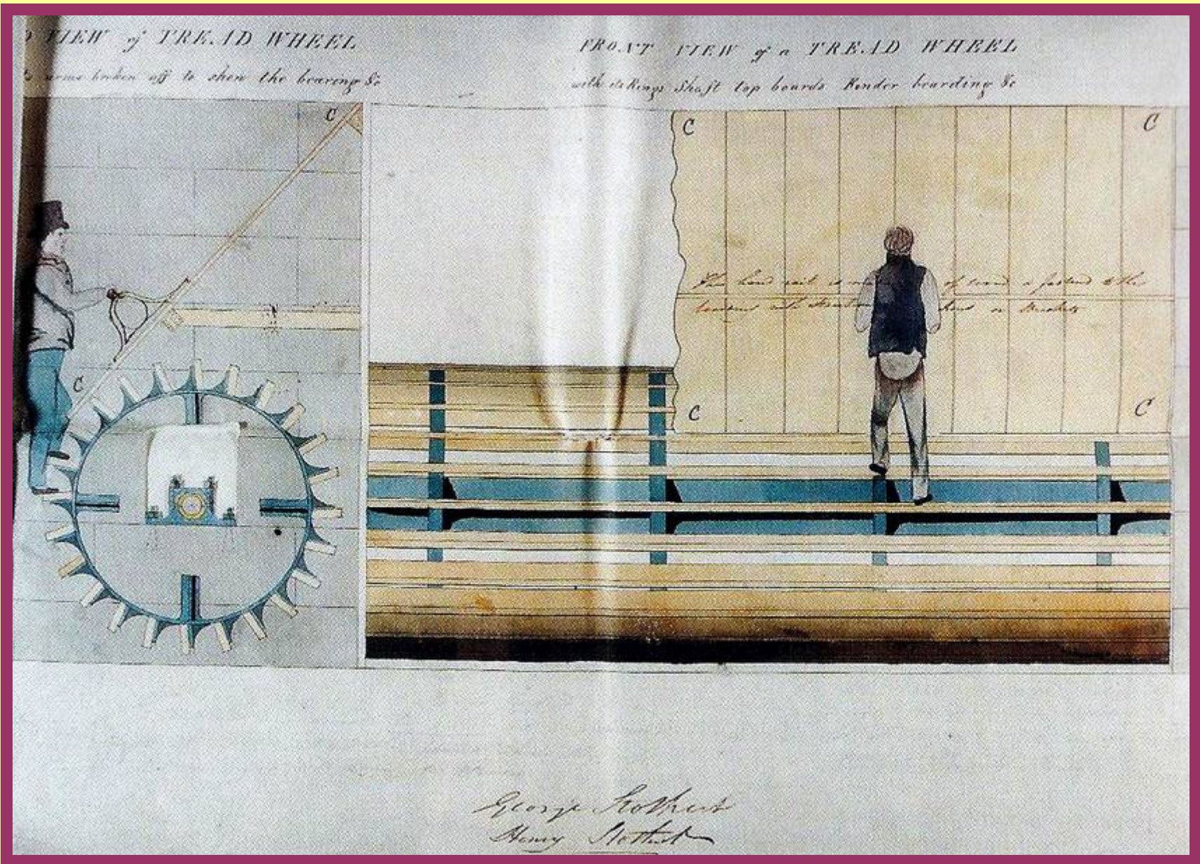
Design for a prison treadmill for Devizes County Gaol by Stothert of Bath, 1823
