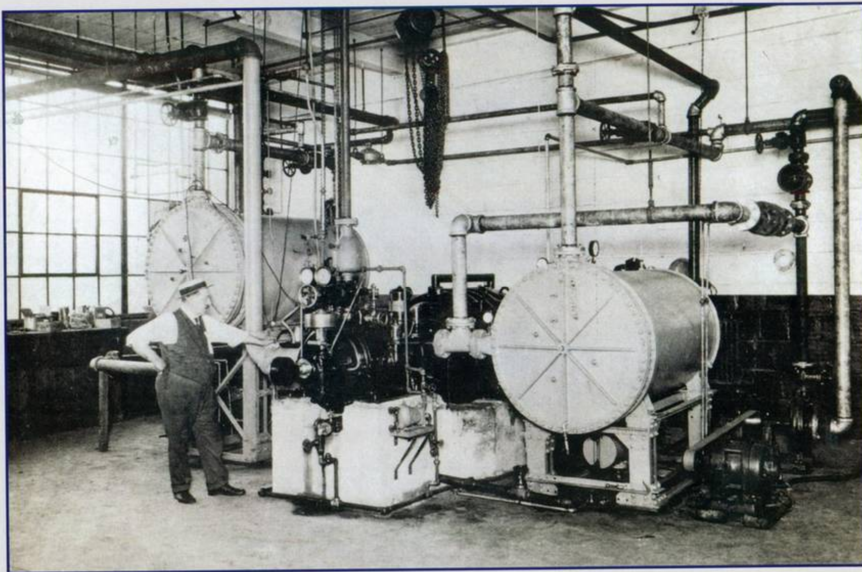
Carrier prototype centrifugal water chiller, Newark, 1922
