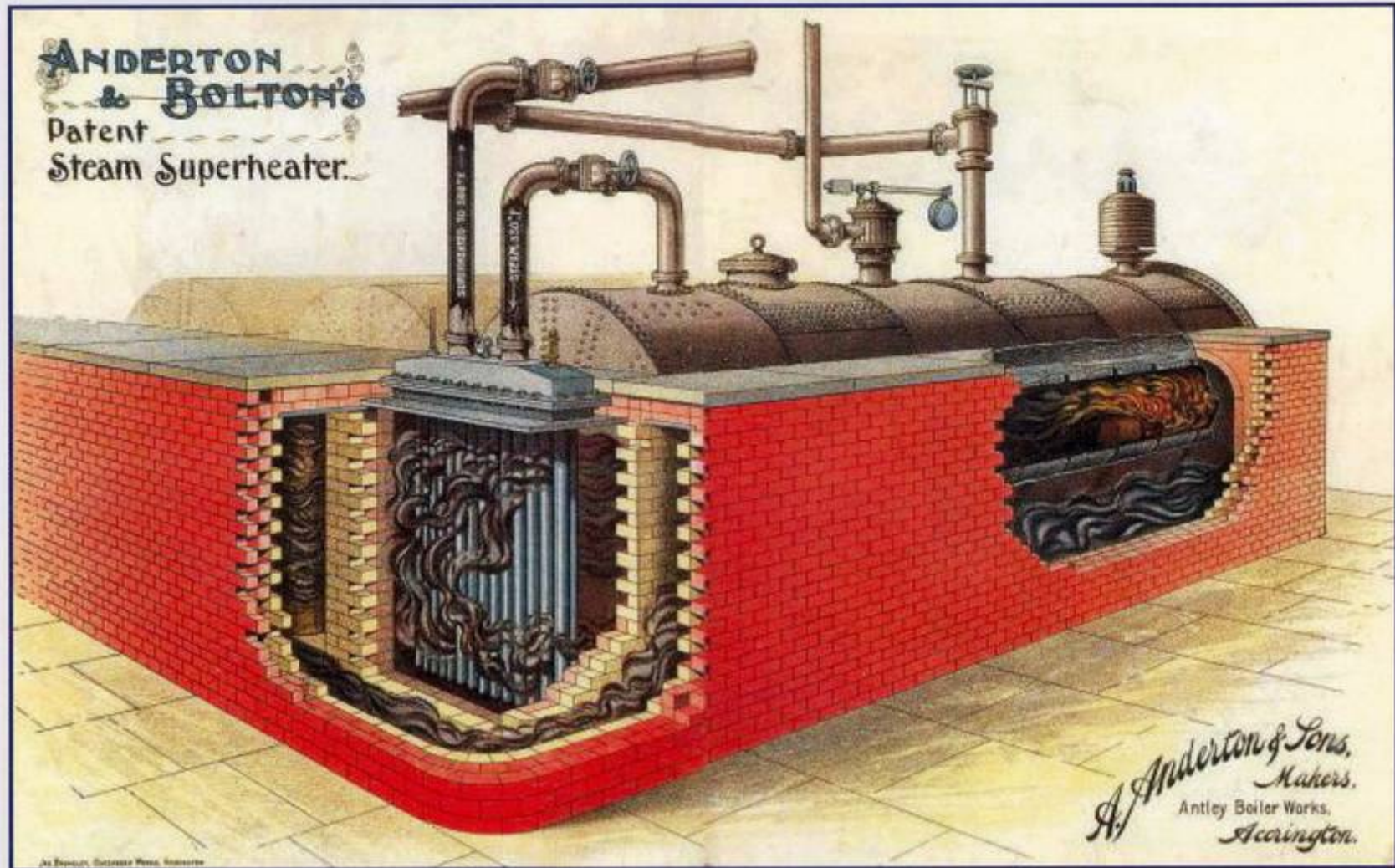
Steam boiler with superheater 1900
