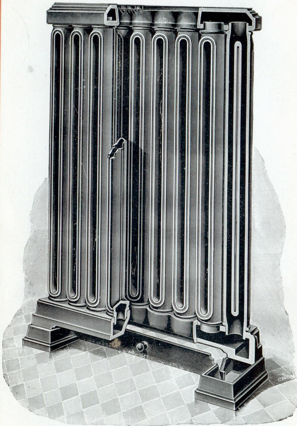
VENTILATING RADIATOR.
