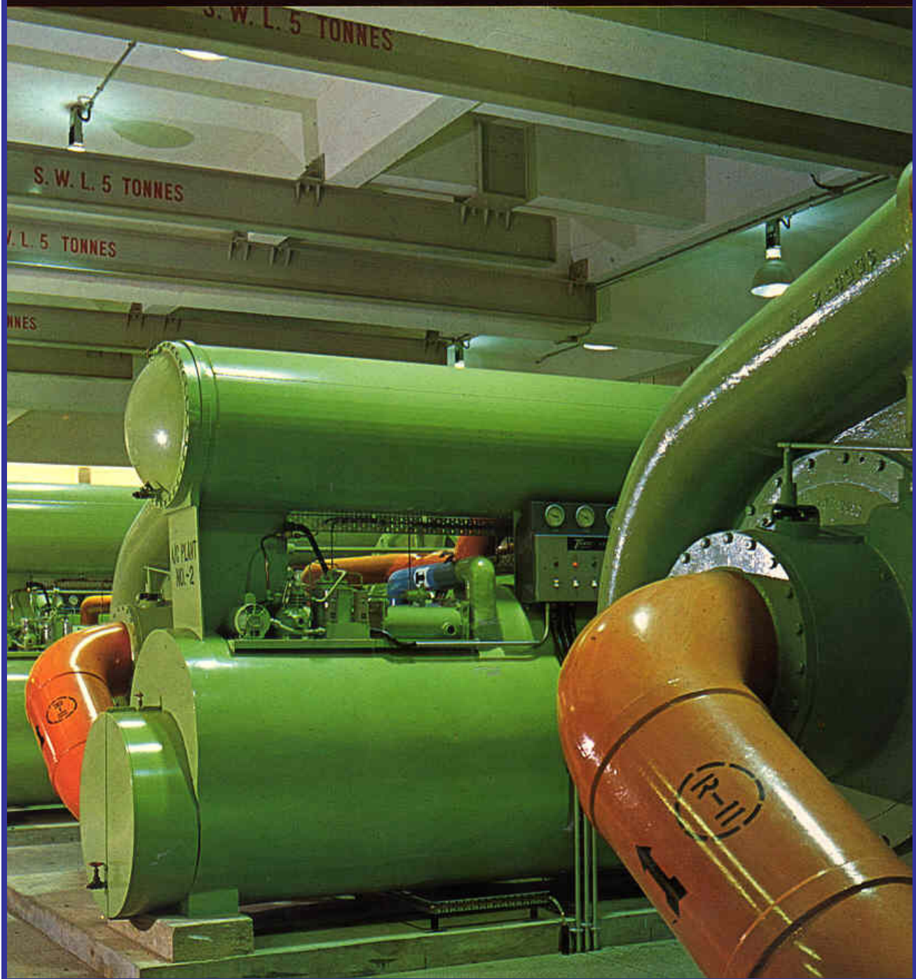
Water chillers at Kai Tak airport, Hong Kong
