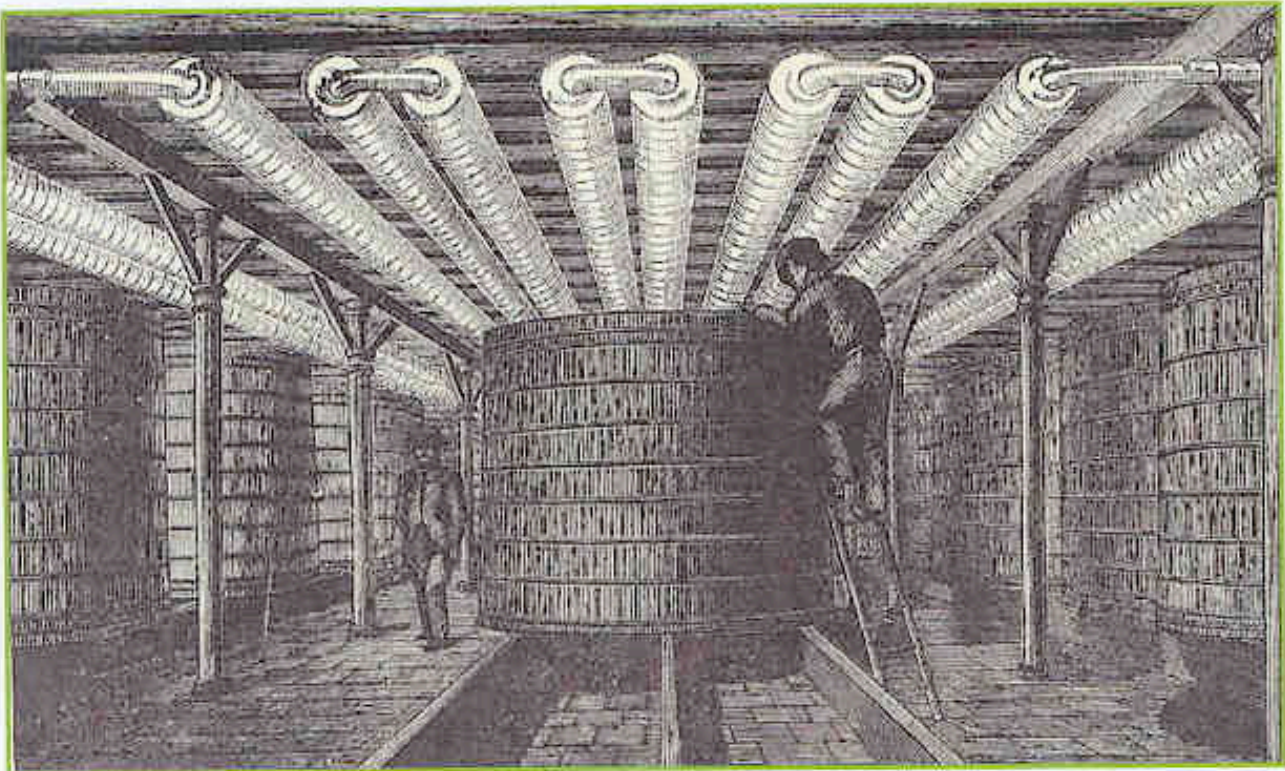
Fermenting room with De La Vergne patent pipe system [Refrigerating and Ice-Making Machinery, 1902, fig.72]
