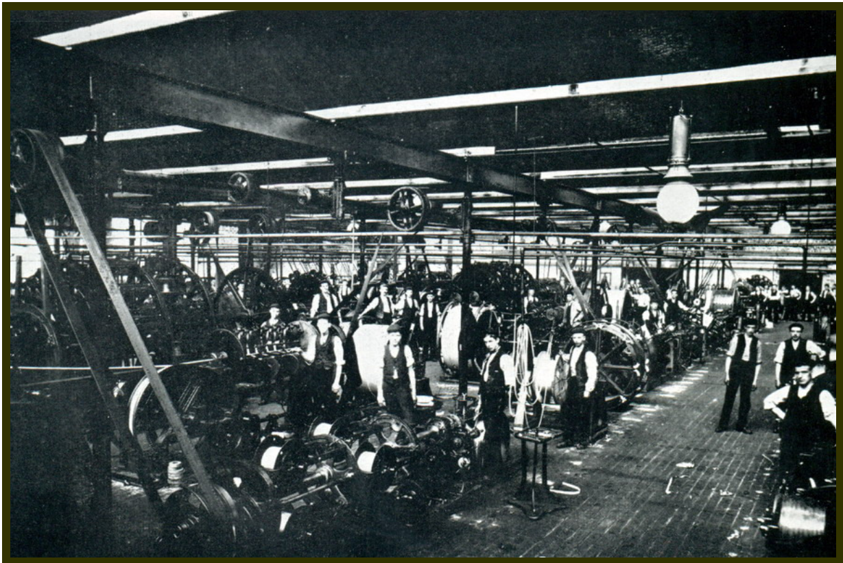
Cable manufacturing at the Prescott Works of the B I Wire Co in 1899 “Electric Cables in Victorian Times,” R M Black, Science Museum, 1972 (CIBSE Heritage Group Collection)
