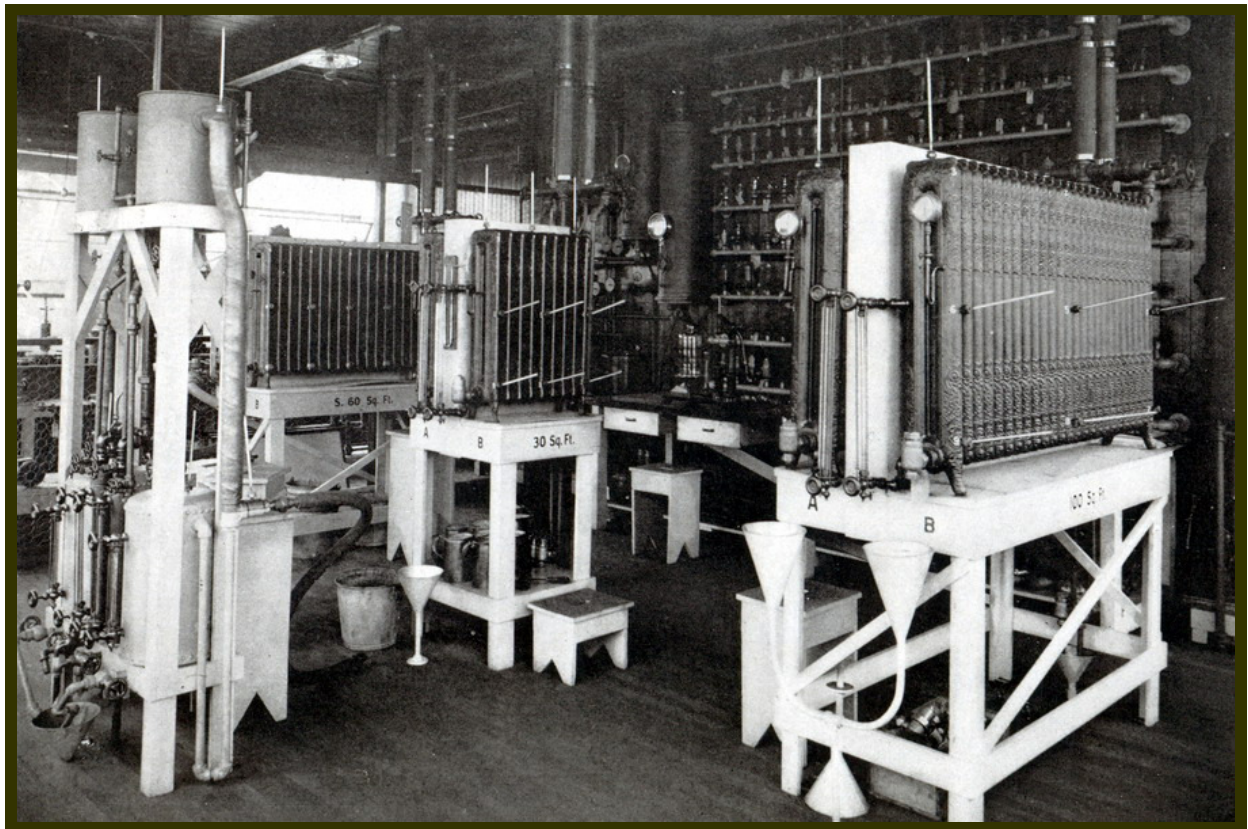
Testing steam traps at Warren Webster & Co, Camden, NJ, 1922 “Steam Heating,” Warren Webster, 1922 (CIBSE Heritage Group Collection)
