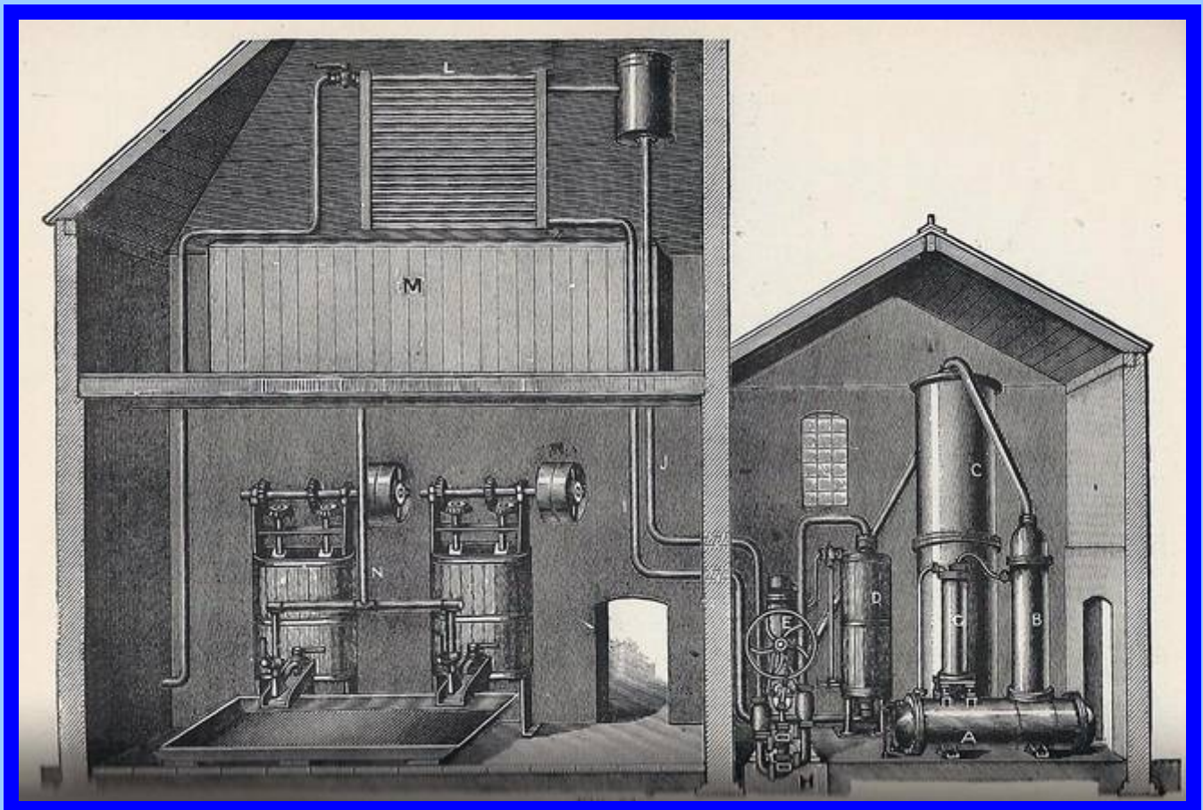
Ammonia absorption refrigeration serving an artificial butter factory
