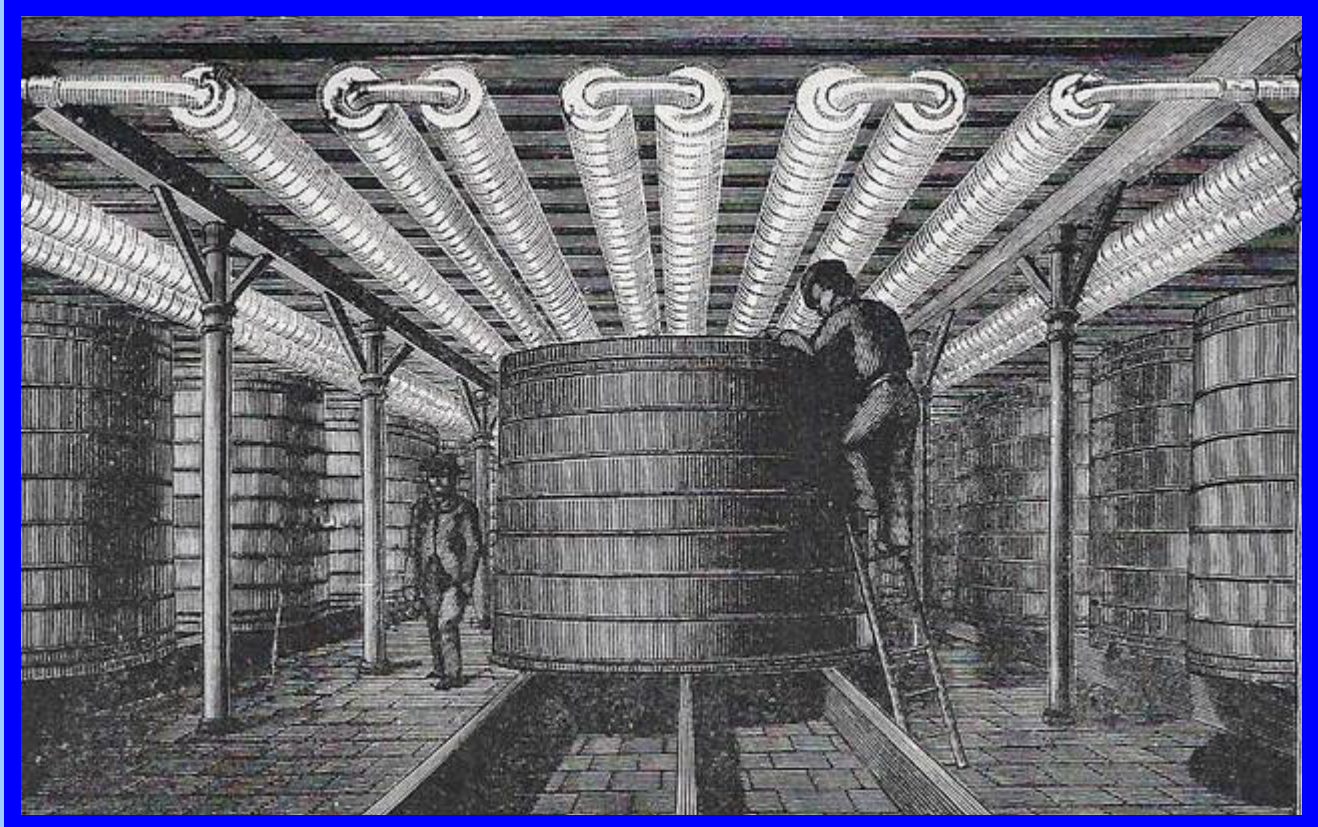
Cooling a fermenting room by De La Vergne system, 1902 book
