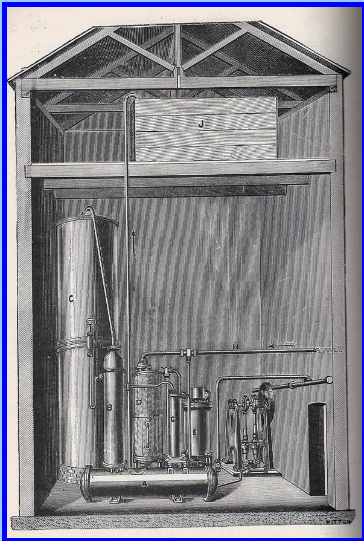
Pontifex-Wood ammonia absorption machine 1902
