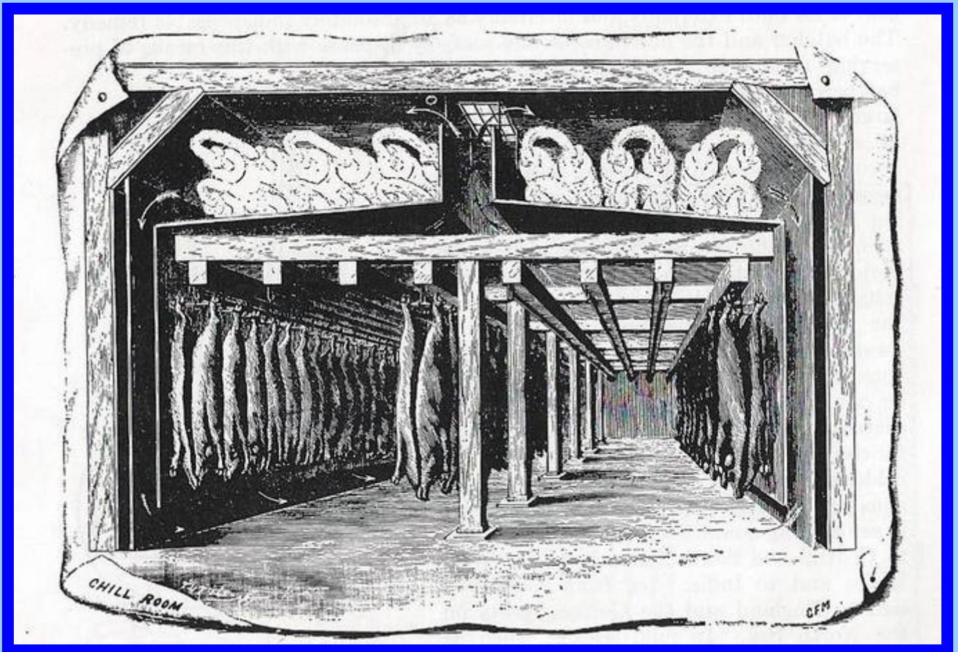
American woodcut of cold store from an 1890 De La Vergne catalogue. Note the cast-iron disks, serving as fins, on the cooling coils.
