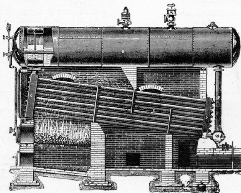
Fig. 132.—WATER TUBE BOILER (Messrs HORNSBY).
