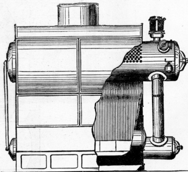
Fig. 123.—WATER TUBE BOILER, Larger Type (Messrs THORNYCROFT).
