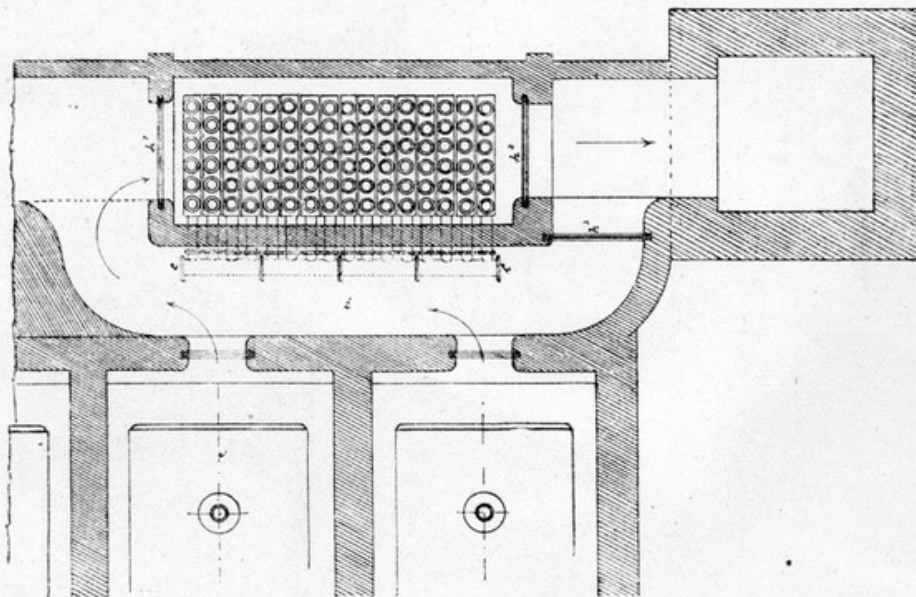
Fig. 140.—Plan of GREEN'S ECONOMISER.
