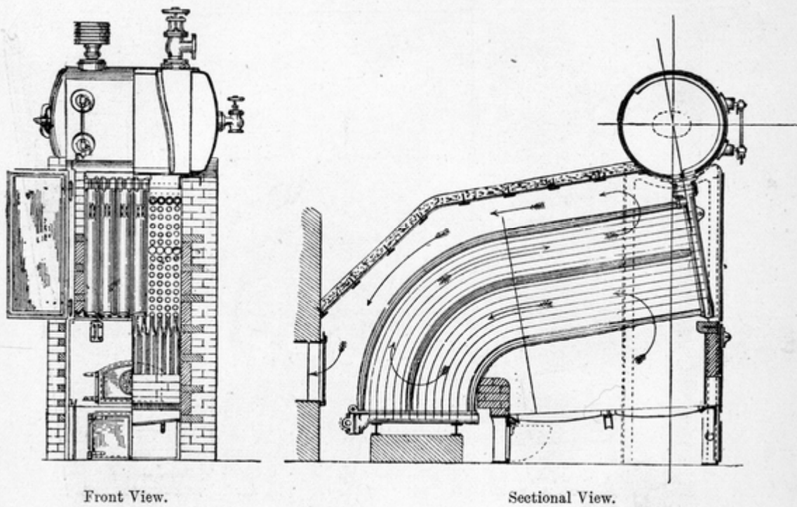
Fig. 134.—HAYTHORN TUBULOUS BOILER.
