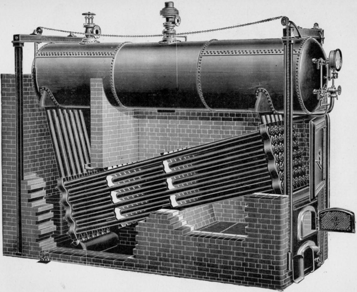
EXAMPLE OF MODERN WATER TUBE BOILER.
