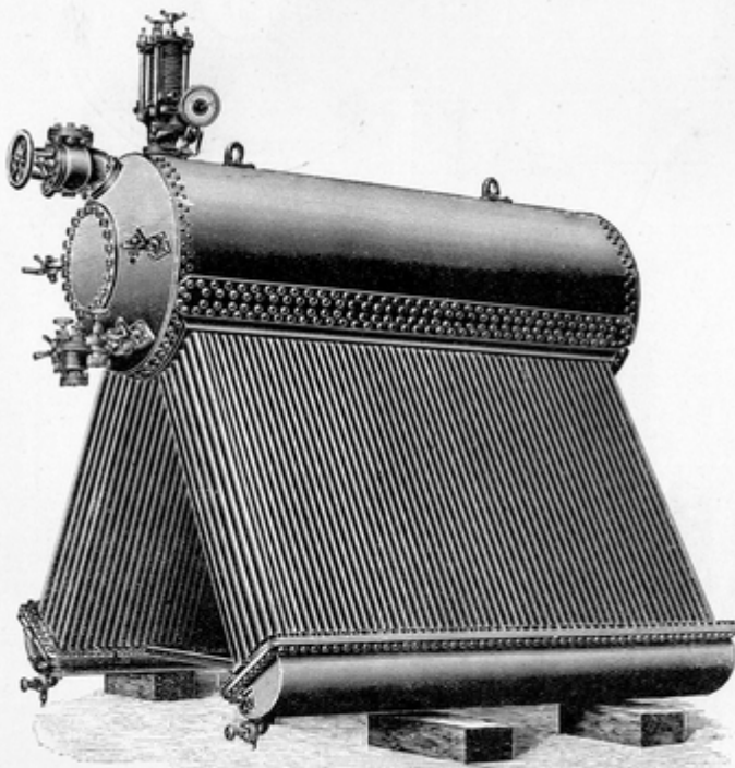
Fig. 124.—“YARROW” WATER TUBE BOILER. Straight Small Tubes.
