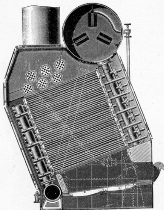
Fig. 131.—WATER TUBE BOILER (Messrs CLARKE CHAPMAN).
