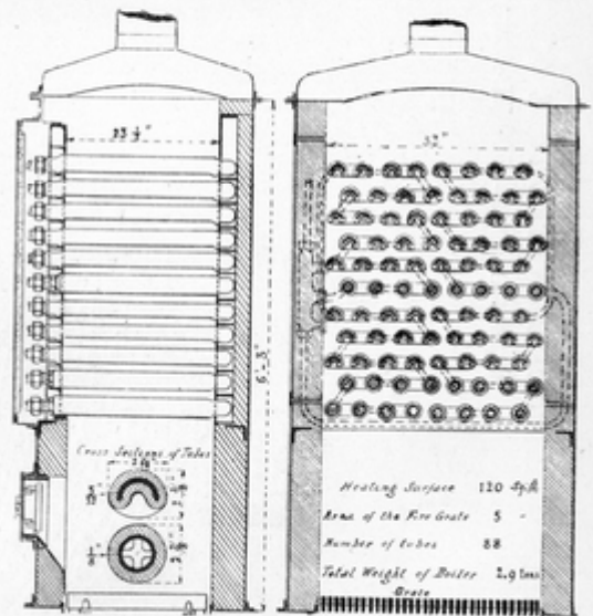
Fig. 125.—“SERPOLLET” BOILER.
