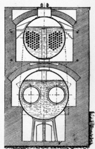
Fig. 120.—Cross Section.
