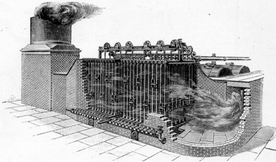
Fig. 139.—Messrs GREEN'S ECONOMISER, for Heating Feed Water by Hot Gases. Vertical 4-inch Tubes, with scrapers.
