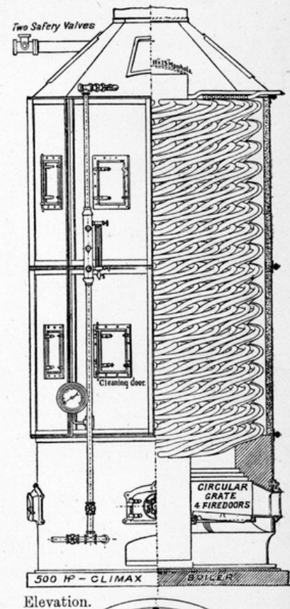
Elevation.
