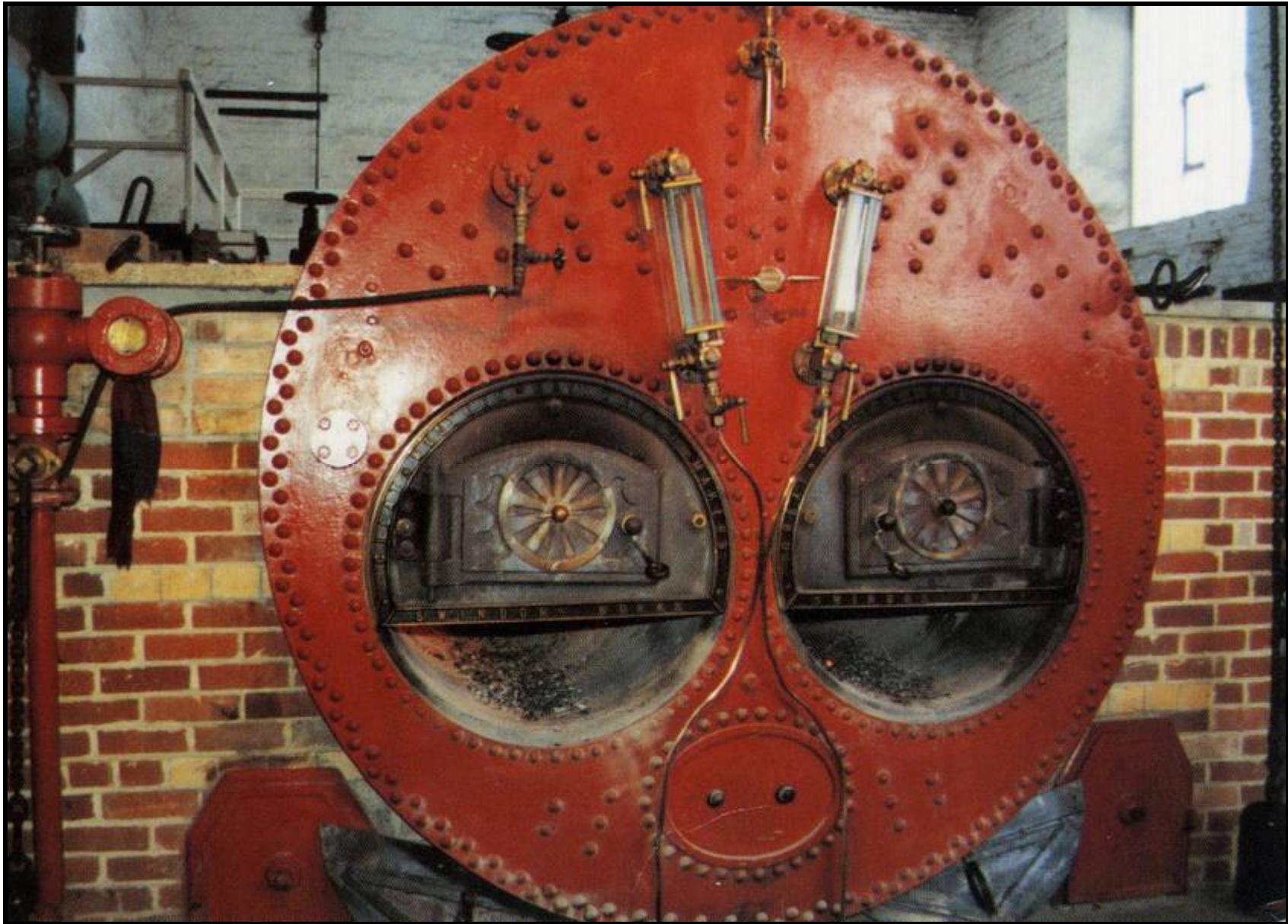
Lancashire Boiler at Crofton Pumping Station
