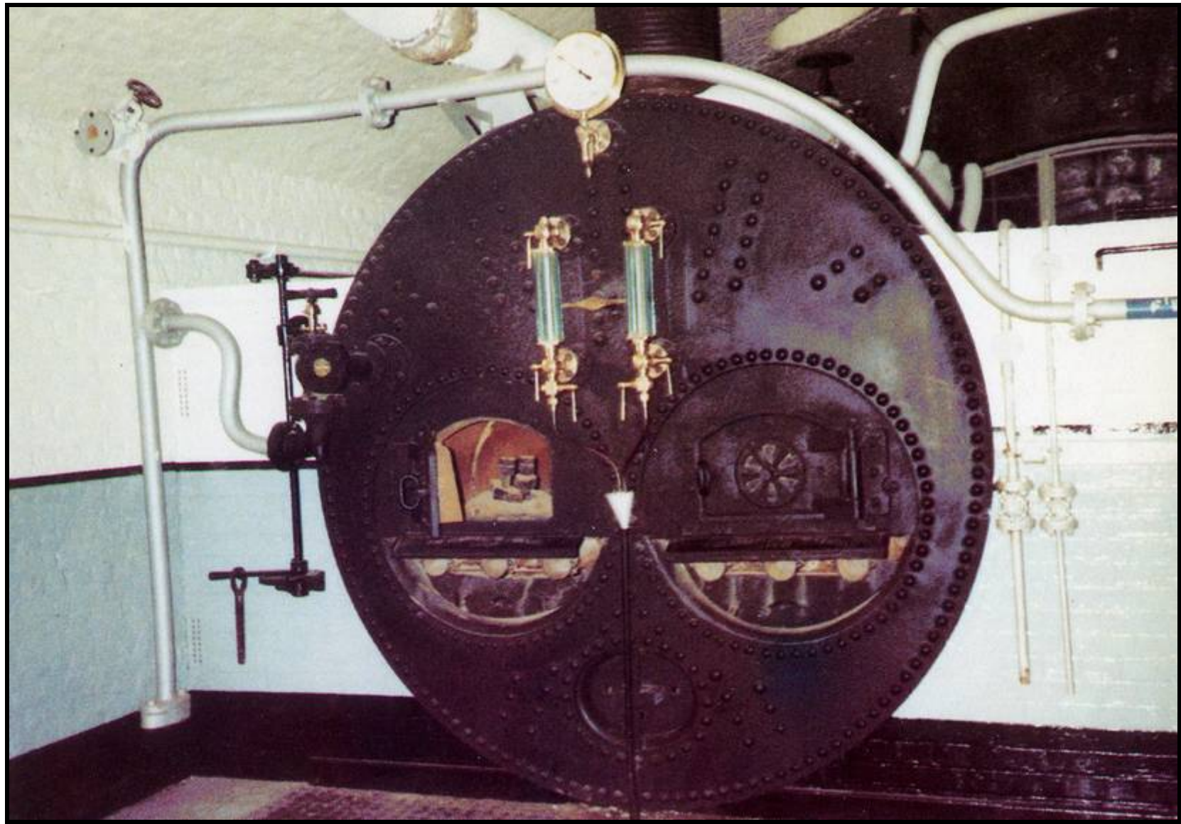
One of the four Boilers serving the Pumping Engines at London's Tower Bridge
