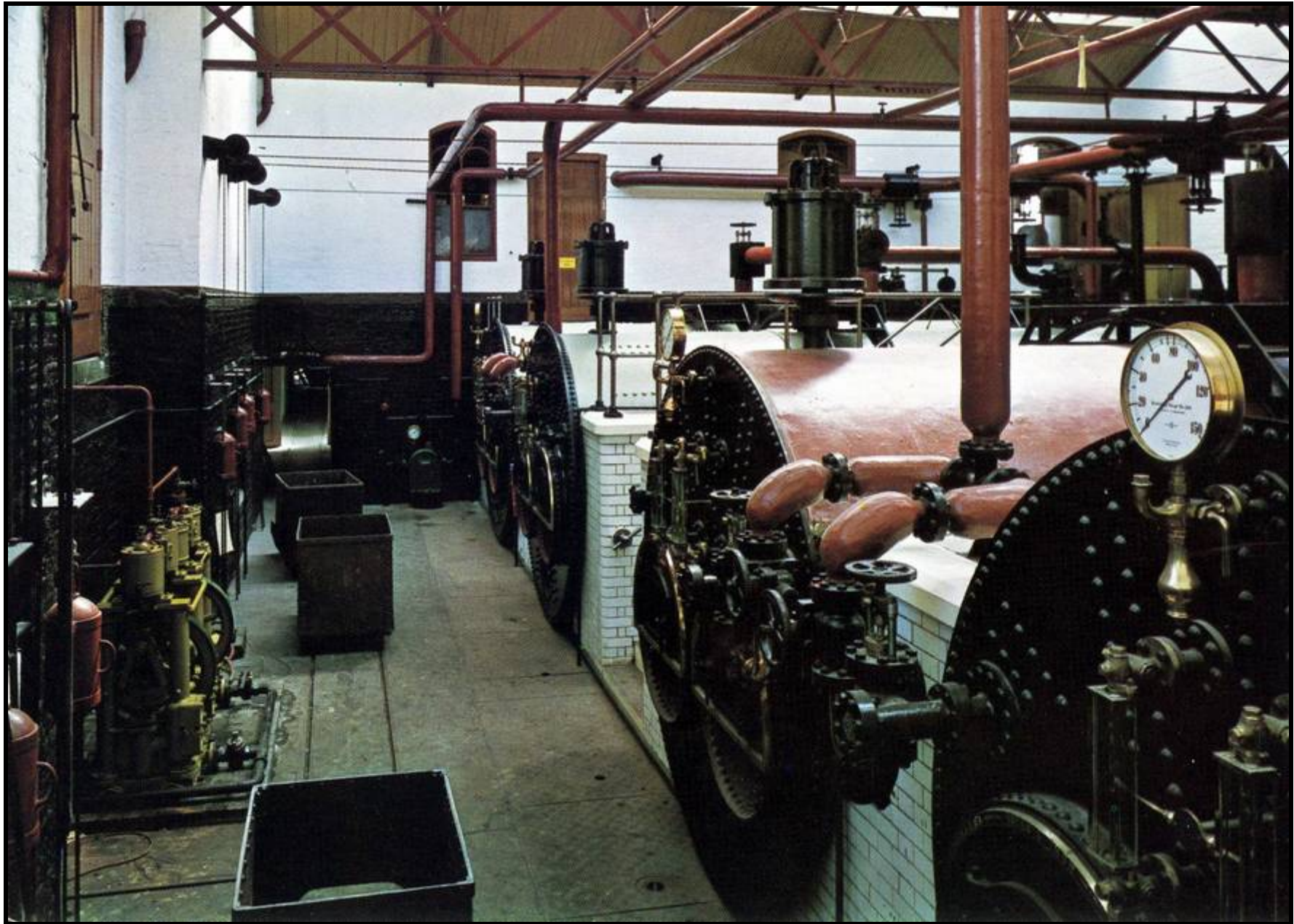
Four Yates & Thom Lancashire Boilers at the Brighton & Hove Engineerium
