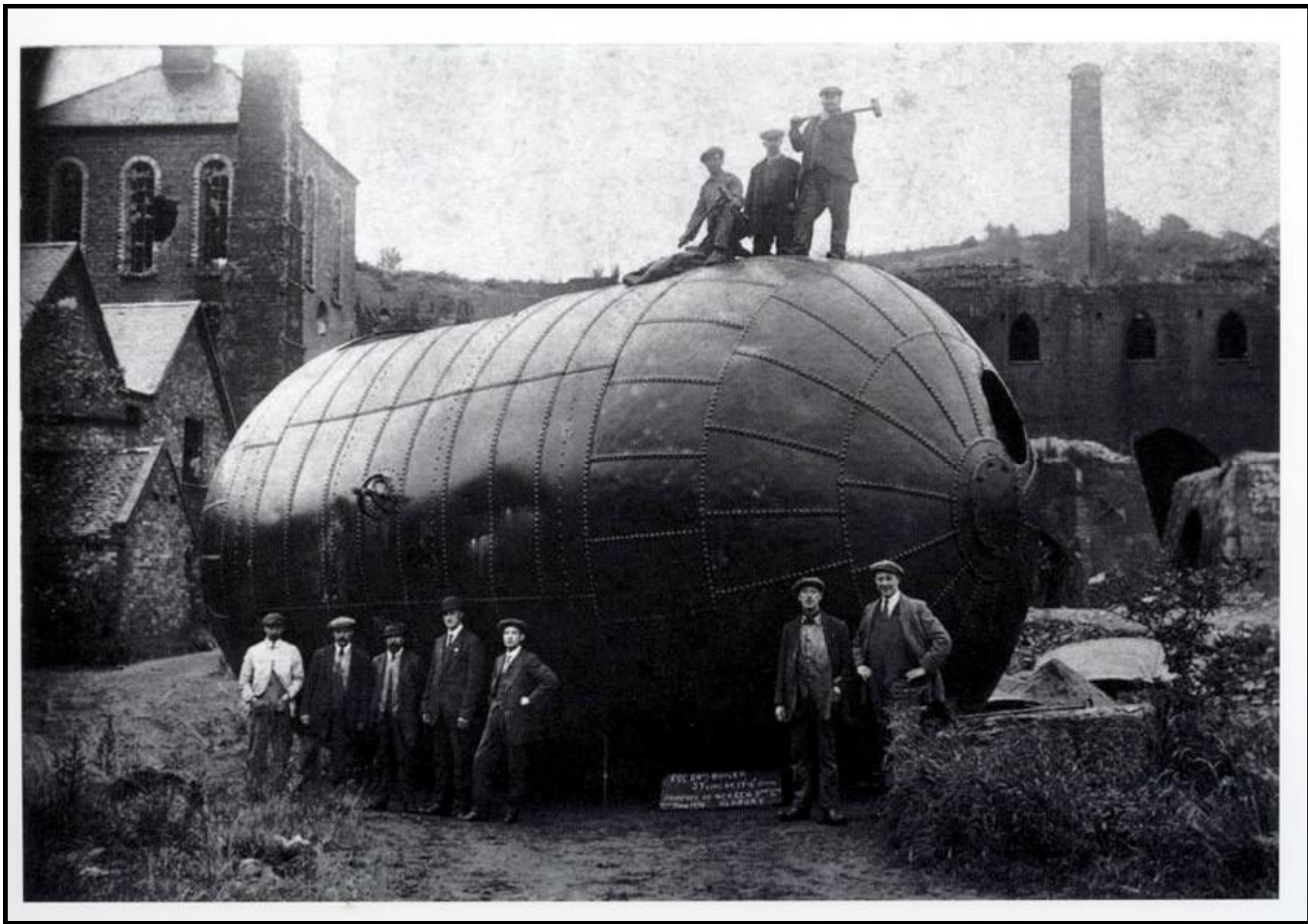
Egg-ended Boiler removed from Blists Hill Blast Furnaces
