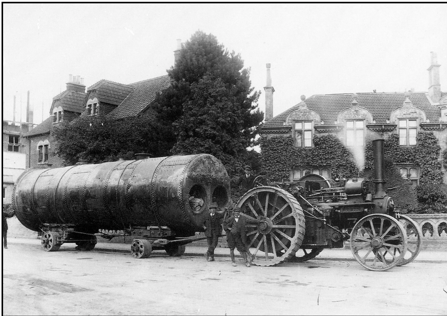
Lancashire Boiler hauled by a Traction Engine in Calne, Wiltshire, c.1919
