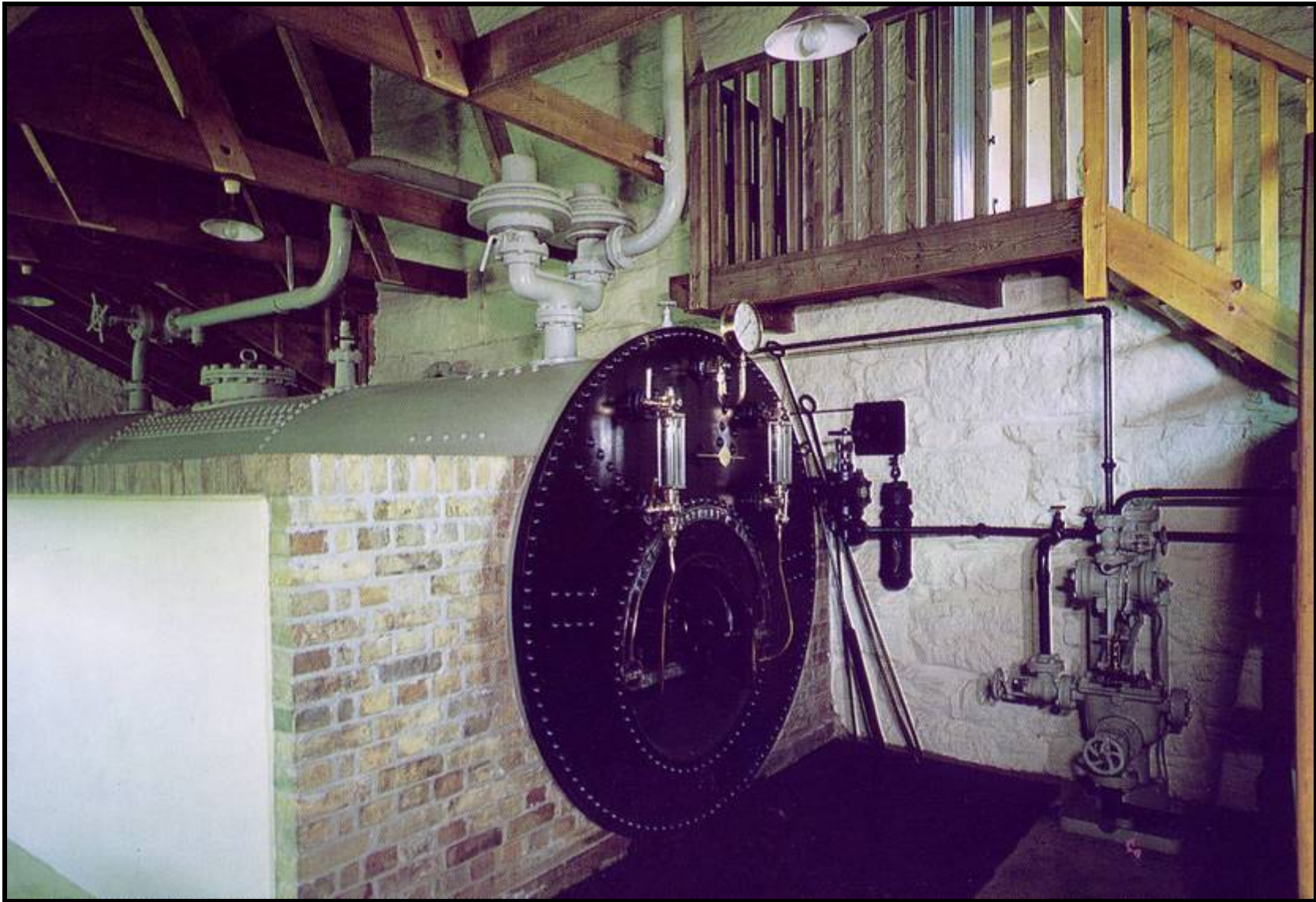
Ruston & Hornsby Cornish Boiler, East Pool Winding Engine, Camborne, Cornwall
