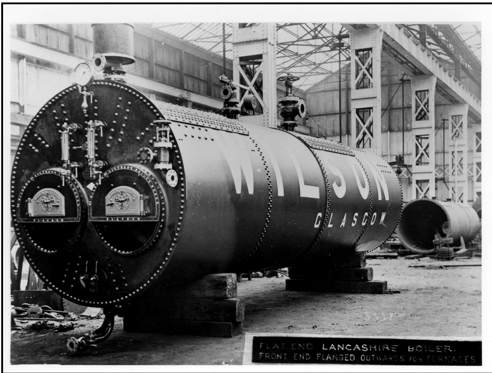
A Lancashire Boiler by William Wilson & Company of Glasgow
